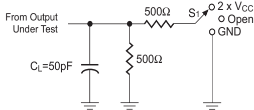
Load Circuit
