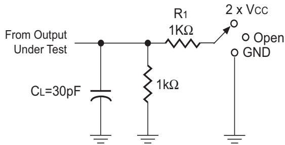
Load Circuit
