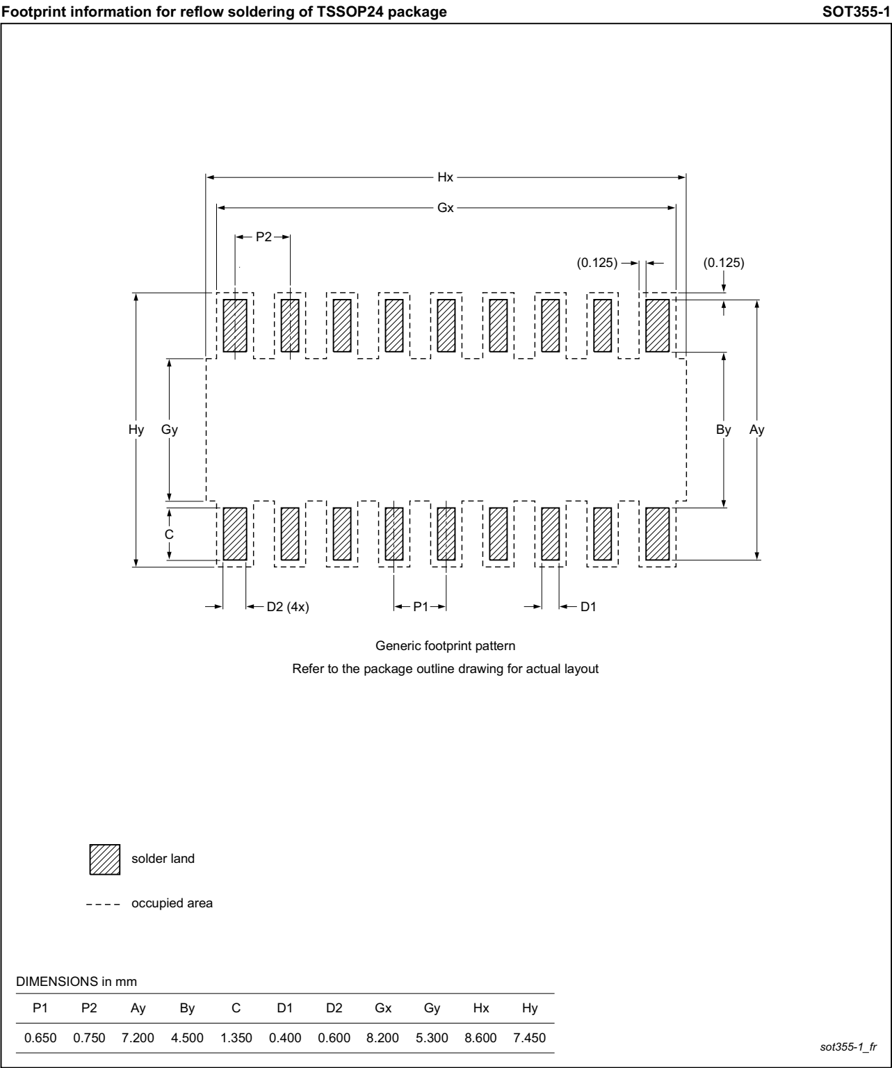
Fig 22. PCB footprint for SOT355-1 (TSSOP24); reflow soldering
