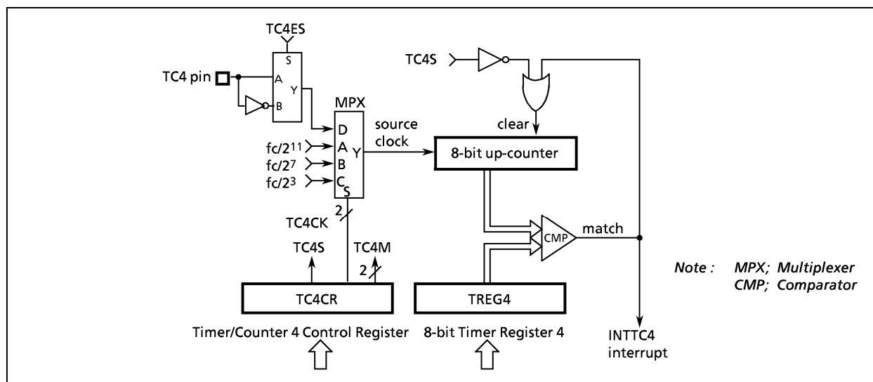
Figure 2-19. Timer/Counter 4
