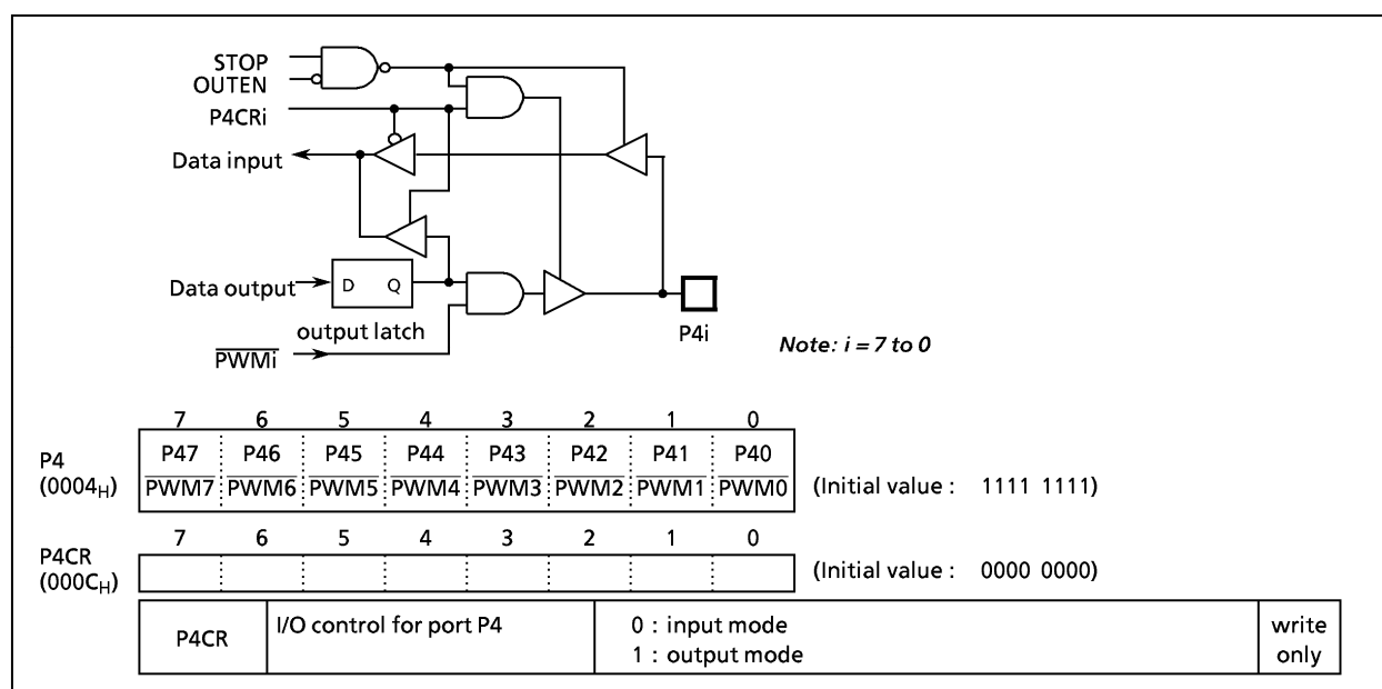
Figure 2-5. Ports P4 and P4CR
