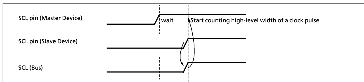
Figure 2-26. Clock Synchronization
