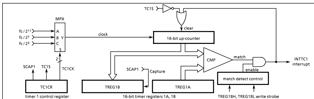
Figure 2-11. Timer 1 (TC1)
