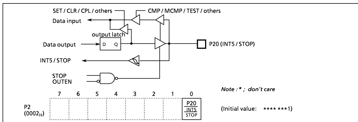
Figure 2-3. Port P2
