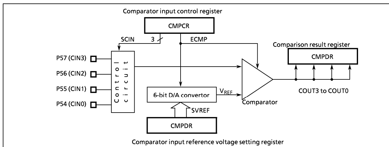
Figure 2-54. 6-bit A/D Conversion (Comparator) Inputs
