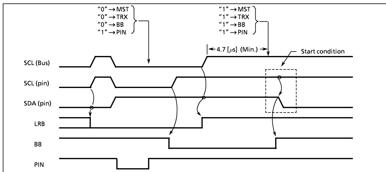
Figure 2-36. Timing Diagram when Restarting
