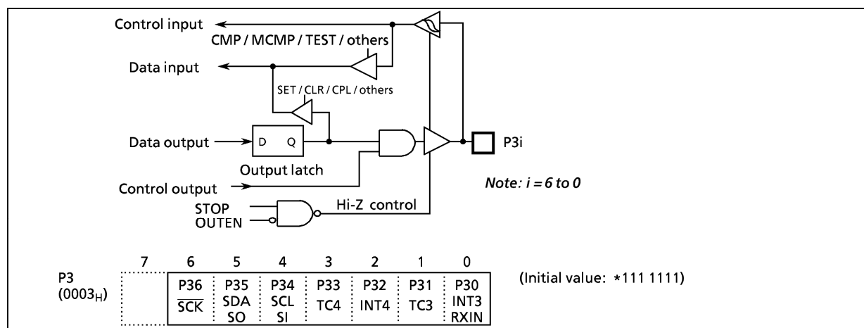
Figure 2-4. Port P3
