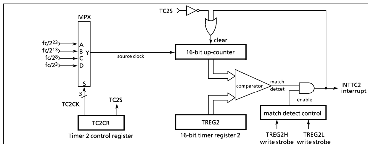
Figure 2-14. Timer 2 (TC2)
