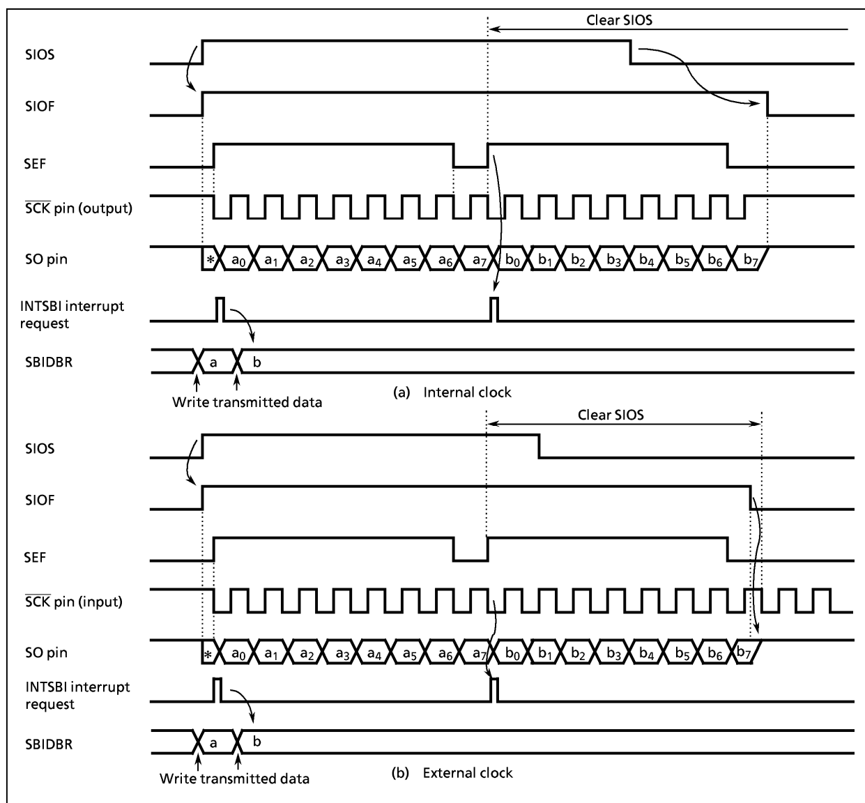
Figure 2-41. Transfer Mode
