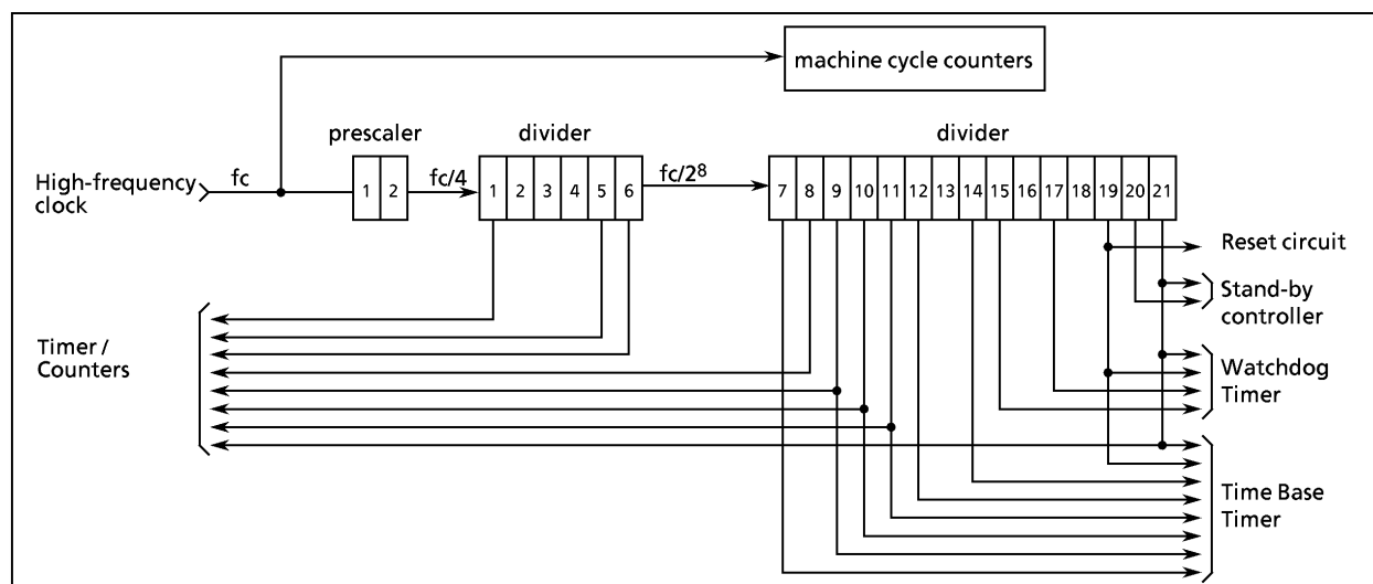
Figure 1-12. Configuration of Timing Generator
