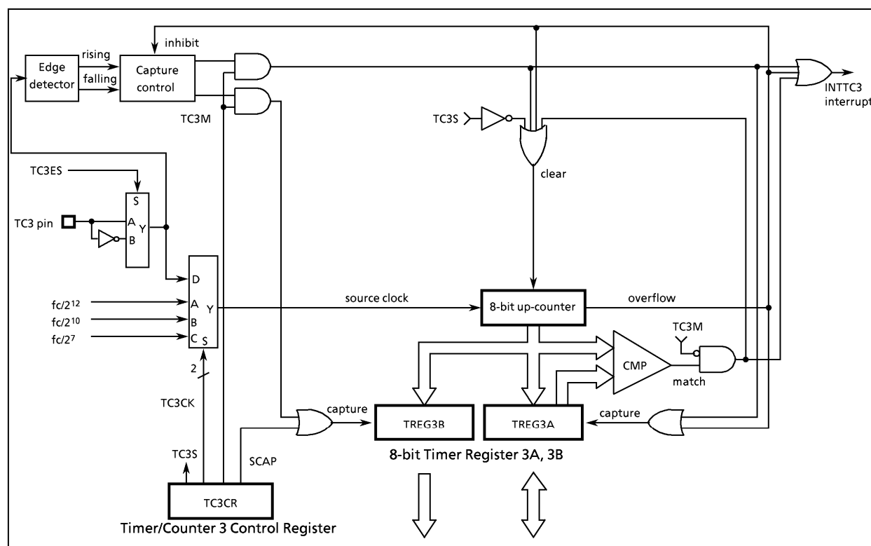
Figure 2-16. Timer/Counter 3
