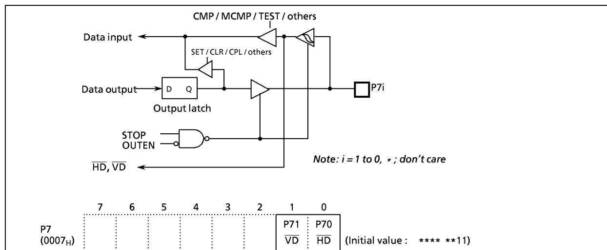
Figure 2-8. Ports P7
