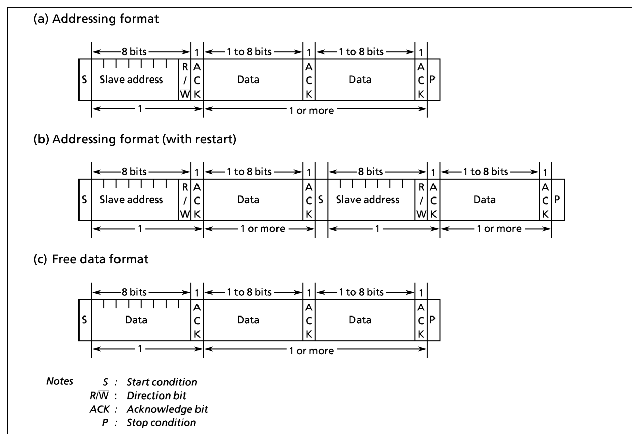
Figure 2-22. Data Format
