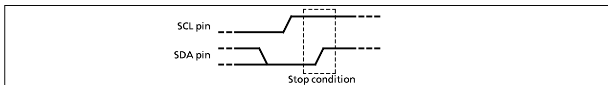
Figure 2-28. Stop Condition Generation
