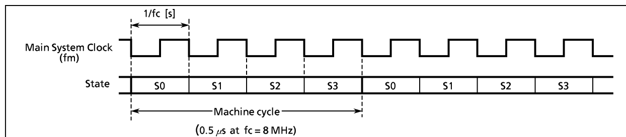
Figure 1-13. Machine Cycle
