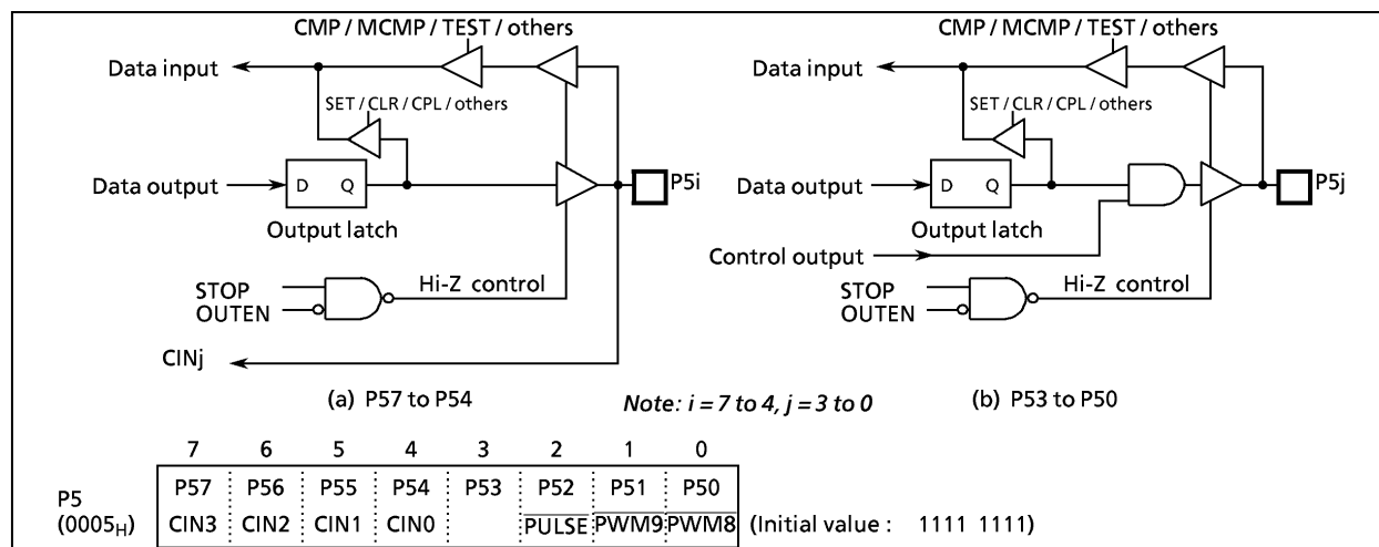
Figure 2-6. Ports P5
