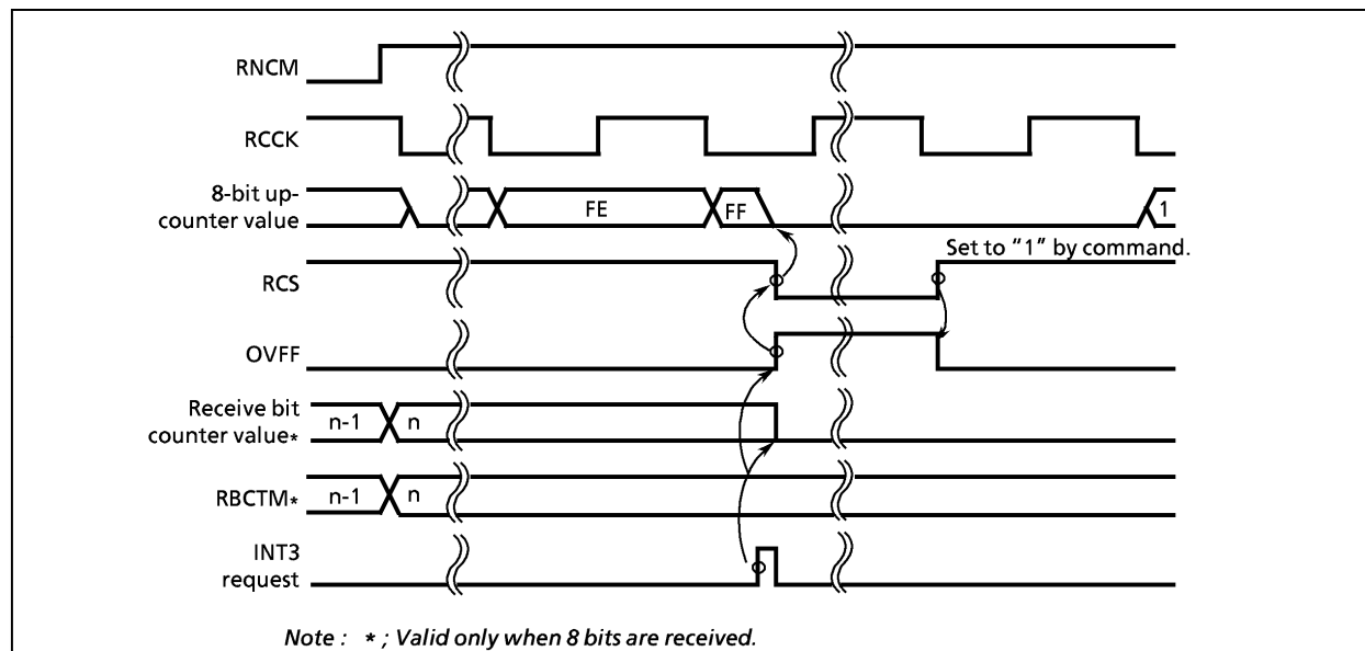
Figure 2-52. Overflow Interrupt Timing Chart
