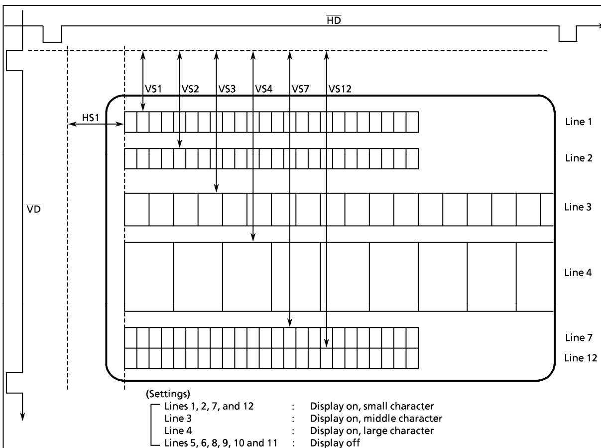
Figure 2-64. TV Screen Image
