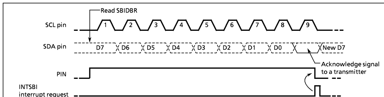
Figure 2-33. Example when BC = "000", ACK = "1" in Receiver Mode
