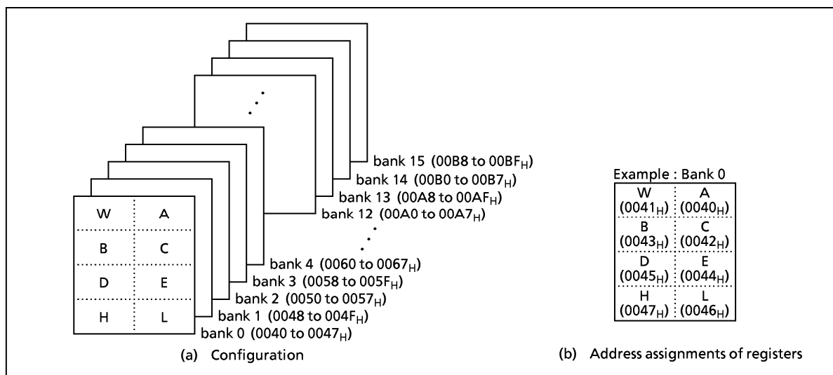
Figure 1-6. General-purpose Register Banks
