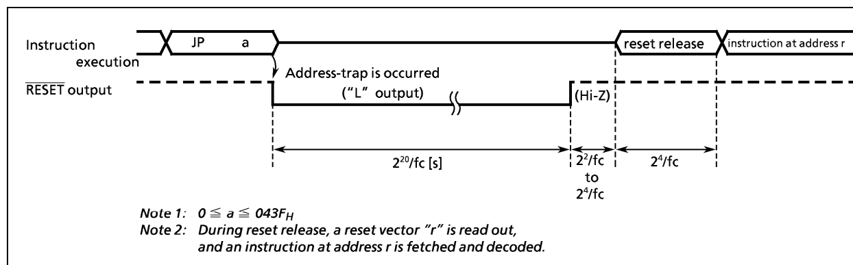
Figure 1-30. Address-Trap-Reset
