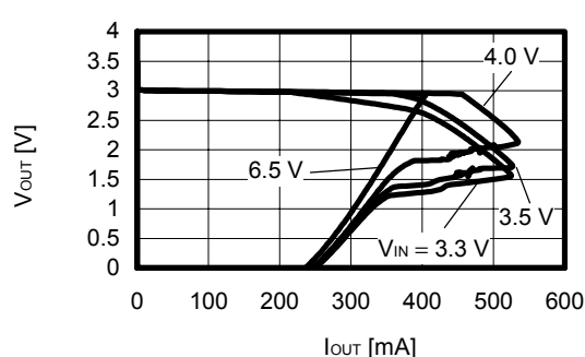
S-1111B30 ( T_a = 25^\circ\text{C} )
