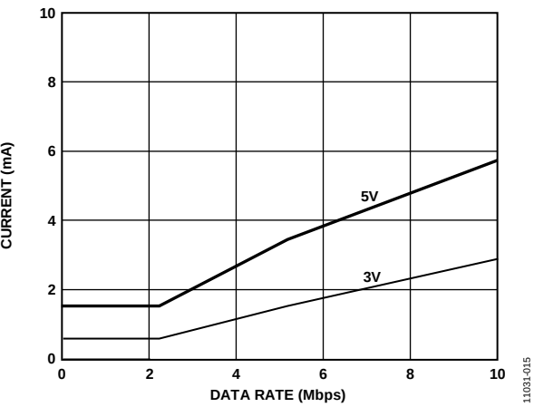
Figure 15. Typical ADuM4402W V_{DD1} or V_{DD2} Supply Current vs. Data Rate for 5 V and 3.3 V Operation
