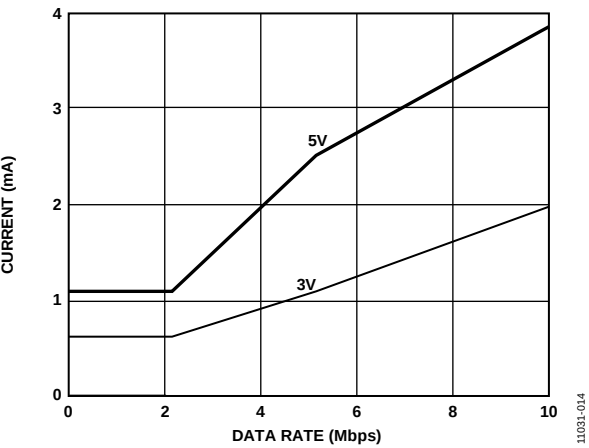
Figure 14. Typical ADuM4401W V_{DD2} Supply Current vs. Data Rate for 5 V and 3.3 V Operation
