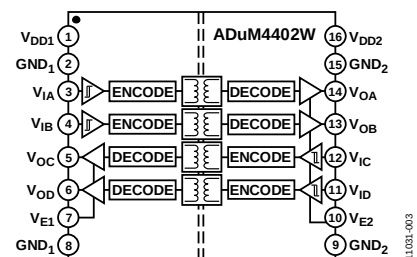
Figure 3. ADuM4402W
