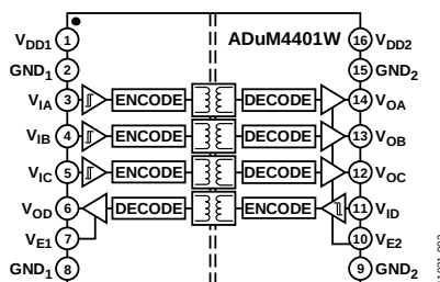
Figure 2. ADuM4401W
