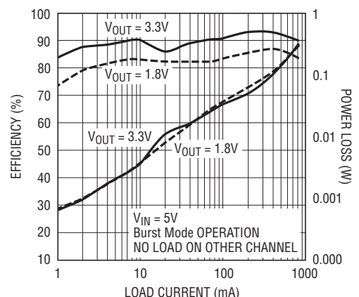
LTC3407-3 Efficiency/Power Loss
