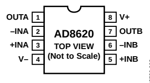
Figure 2. 8-Lead SOIC_N
