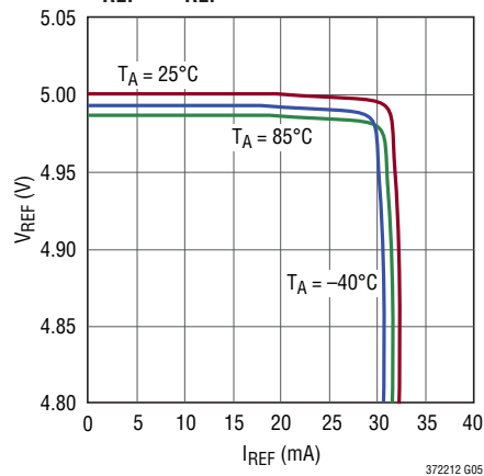
V_{REF} vs I_{REF}
