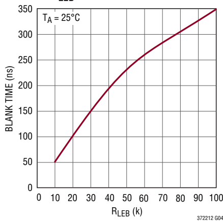
Leading Edge Blanking Time vs R_{LEB}
