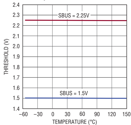
Delay Pin Threshold vs Temperature
