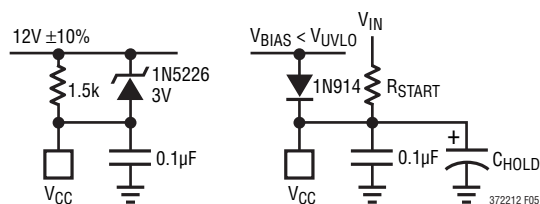
Figure 5. Bias Configurations
