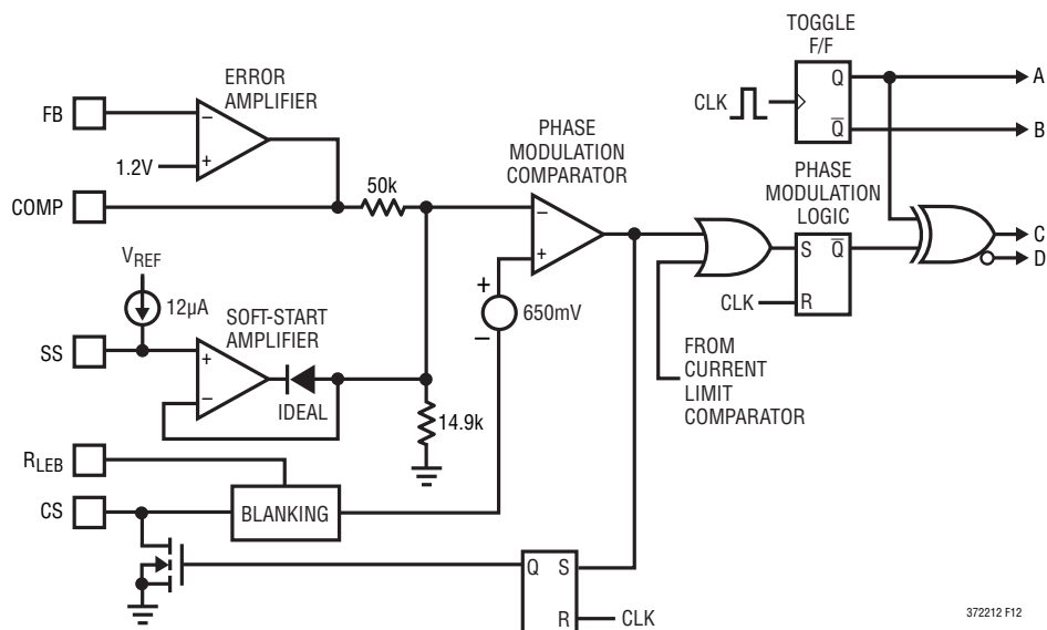
Figure 12. Phase Modulation Circuitry (LTC3722-1)
