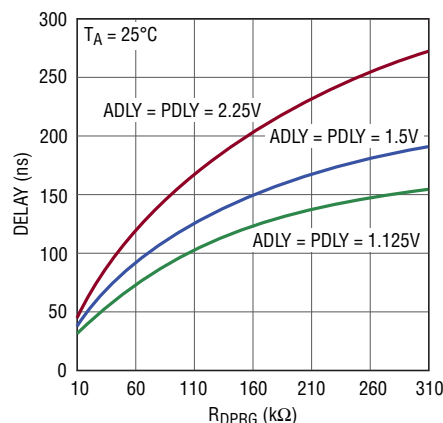
ZVS Delay in Fixed Mode, SBUS = 5V
