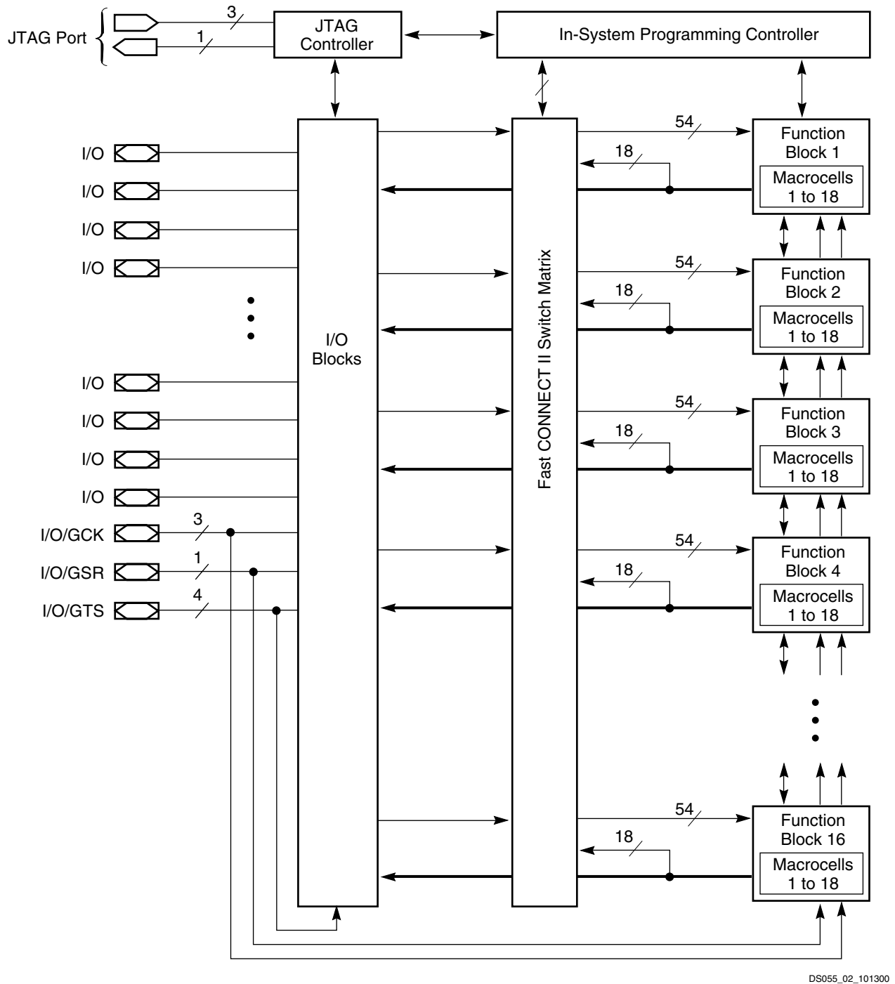
Figure 2: XC95288XL Architecture
