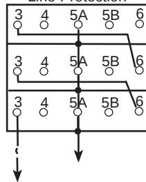
Wiring for Multiple Line Protection
