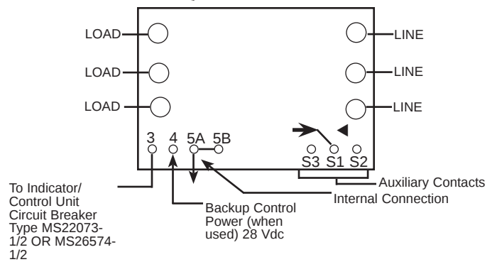
Contacts and Coil Circuits Only
