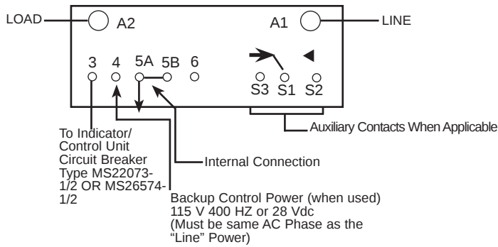
Contacts and Coil Circuits Only
