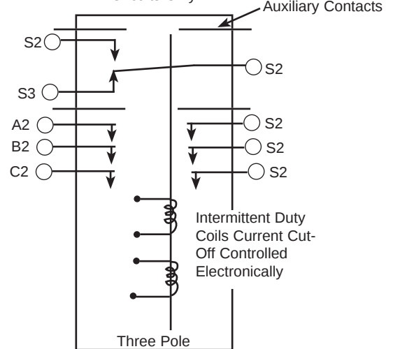
Contacts and Coil Circuits Only
