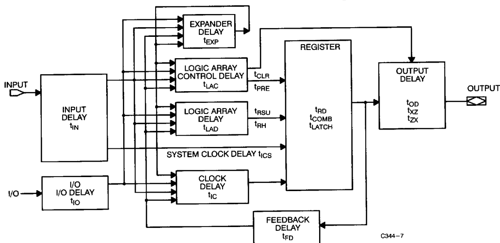
Figure 1. CY7C344/CY7C344B Timing Model
