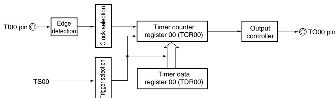
Figure 6-45. Block Diagram of Operation as Frequency Divider
