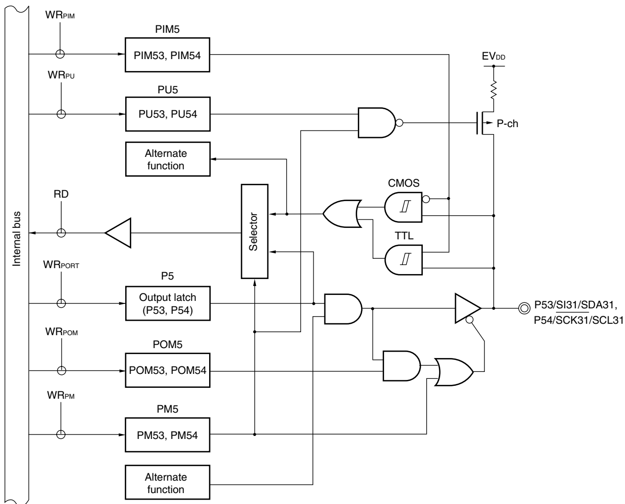
Figure 4-30. Block Diagram of P53, P54
