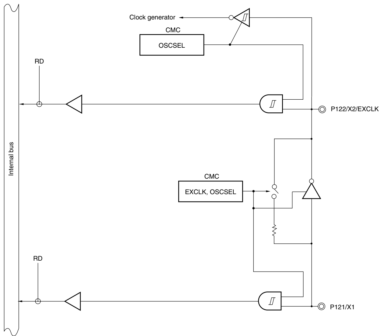
Figure 4-52. Block Diagram of P121 and P122
