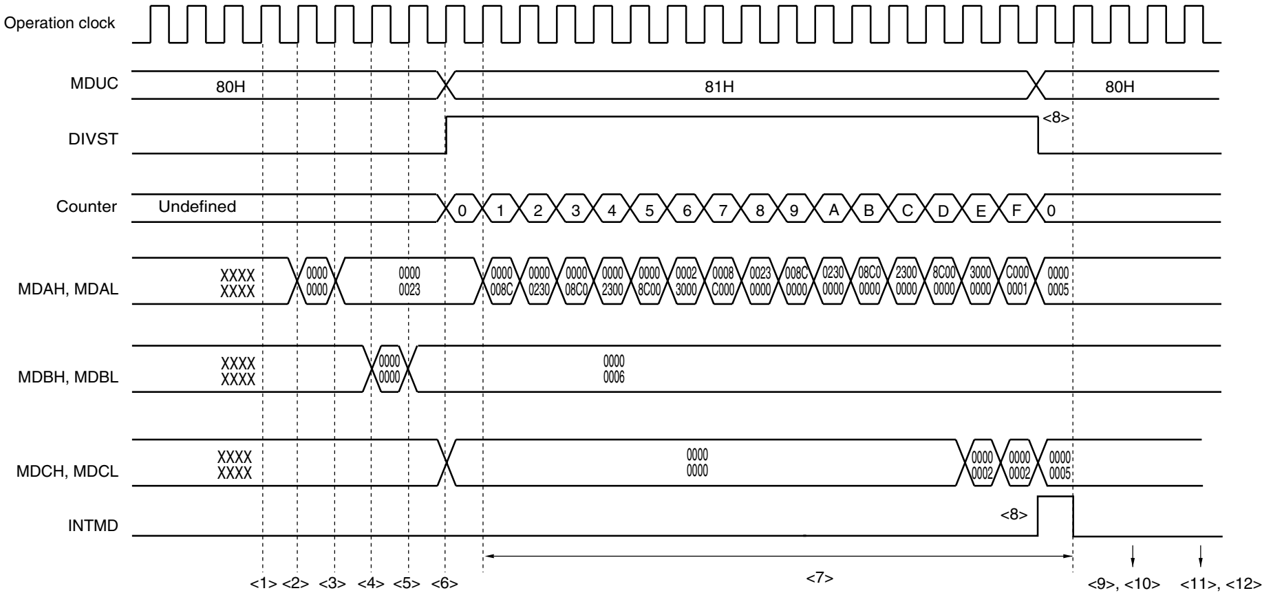
Figure 14-10. Timing Diagram of Division Operation (Example: 35 ÷ 6 = 5, Remainder 5)
