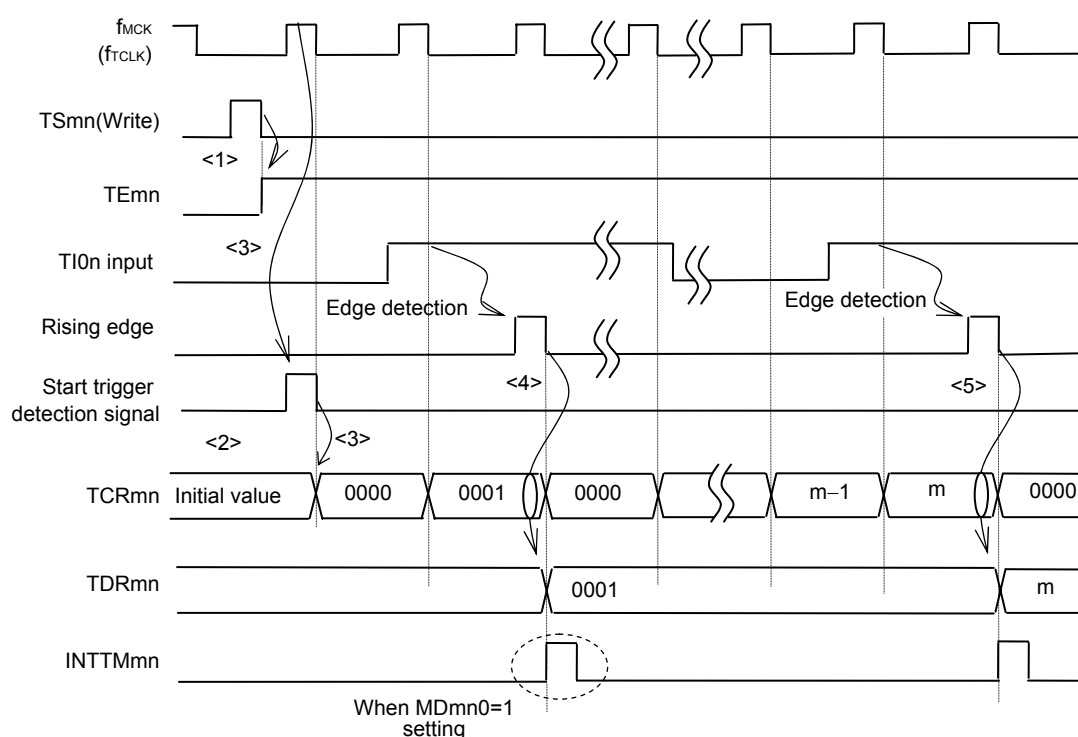
Figure 6-25. Start Timing (In Capture Mode)
