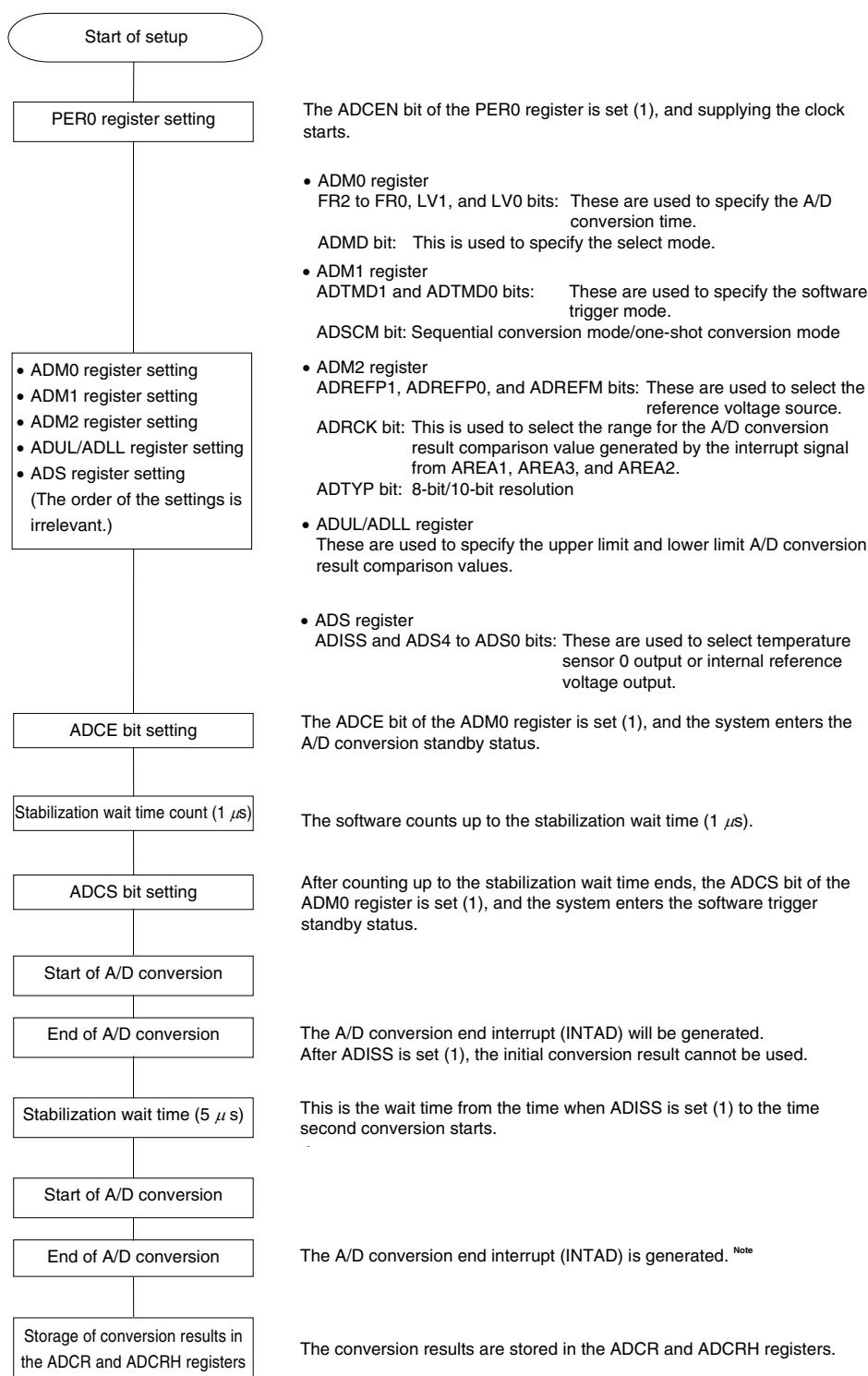
Figure 11-35. Setup When Using Temperature Sensor
