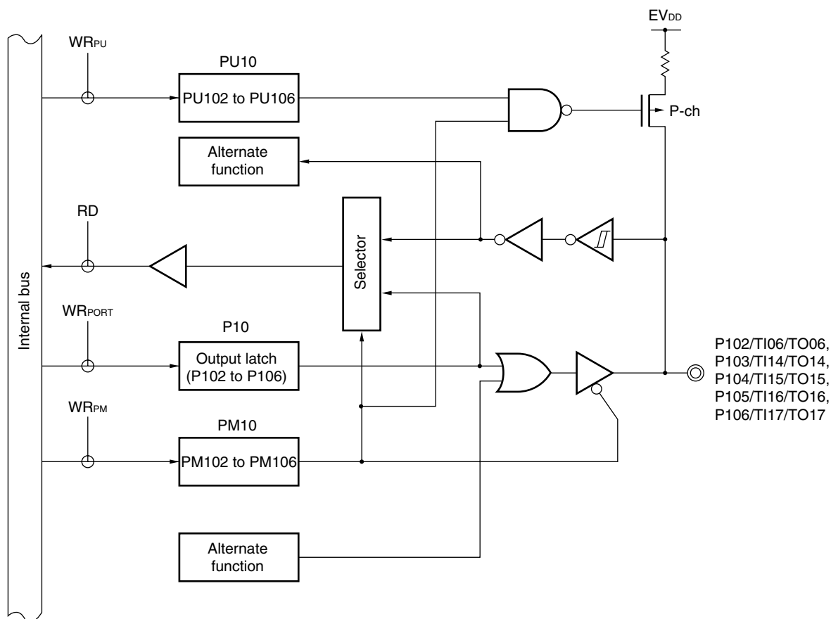
Figure 4-48. Block Diagram of P102 to P106
