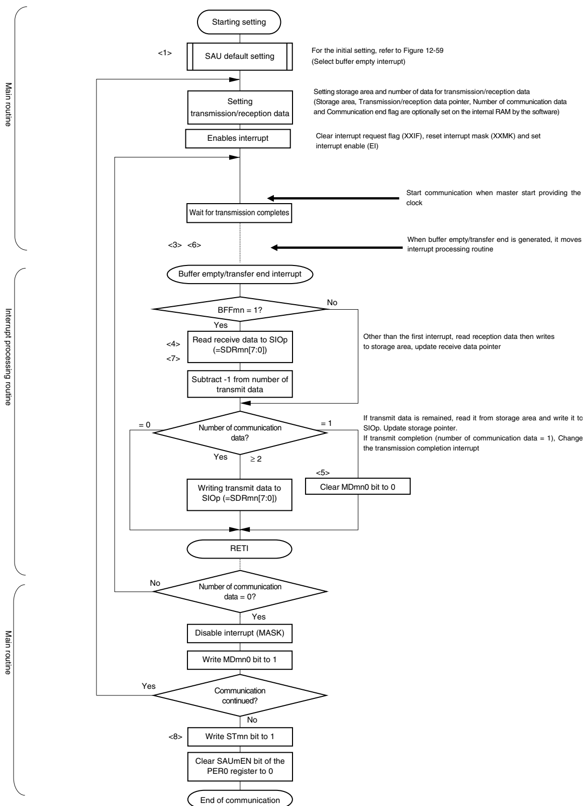
&lt;R&gt; Figure 12-71. Flowchart of Slave Transmission/Reception (in Continuous Transmission/Reception Mode)
