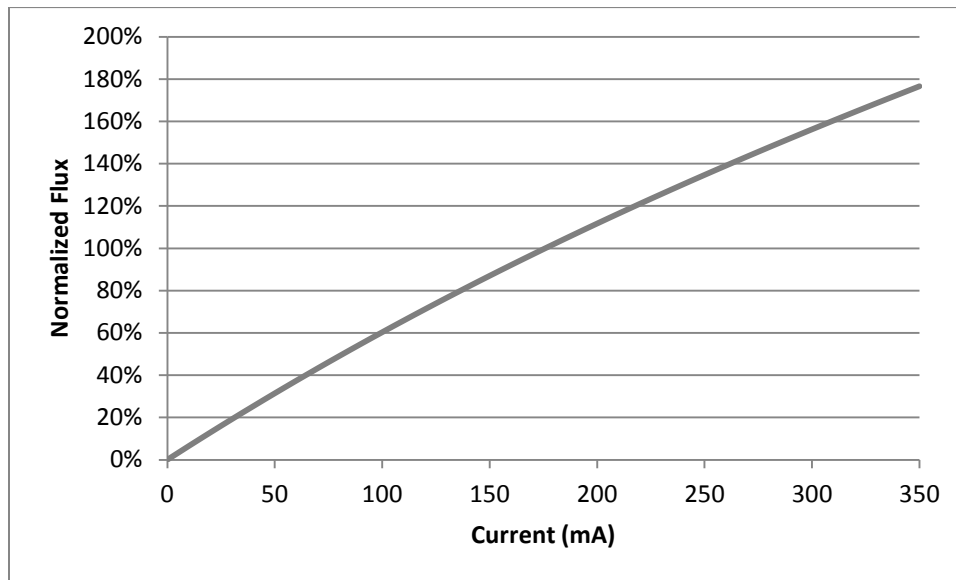
Figure 5: Typical Flux vs. Current – BXRE-xxx-0800-B-xx
