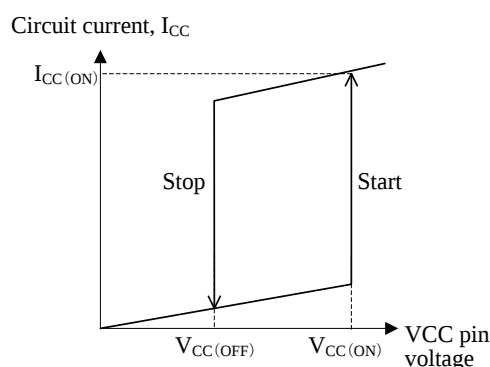
Figure 9-3. Relationship between VCC pin voltage and I_{CC}
