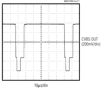
LINE-TIME DISTORTION
