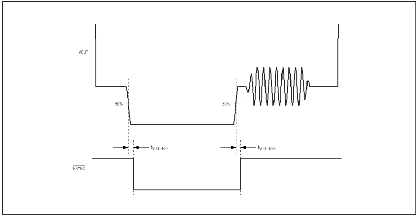
Figure 8. VOUT, and \overline{\text{HSYNC}} Horizontal Sync Timing (NTSC and PAL, External Sync Mode)
