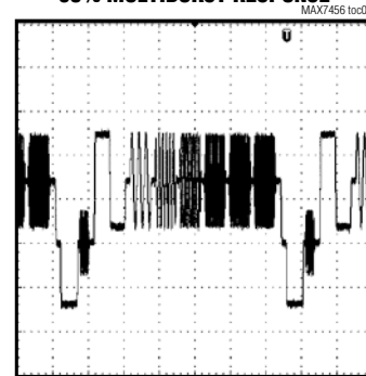
60% MULTIBURST RESPONSE
