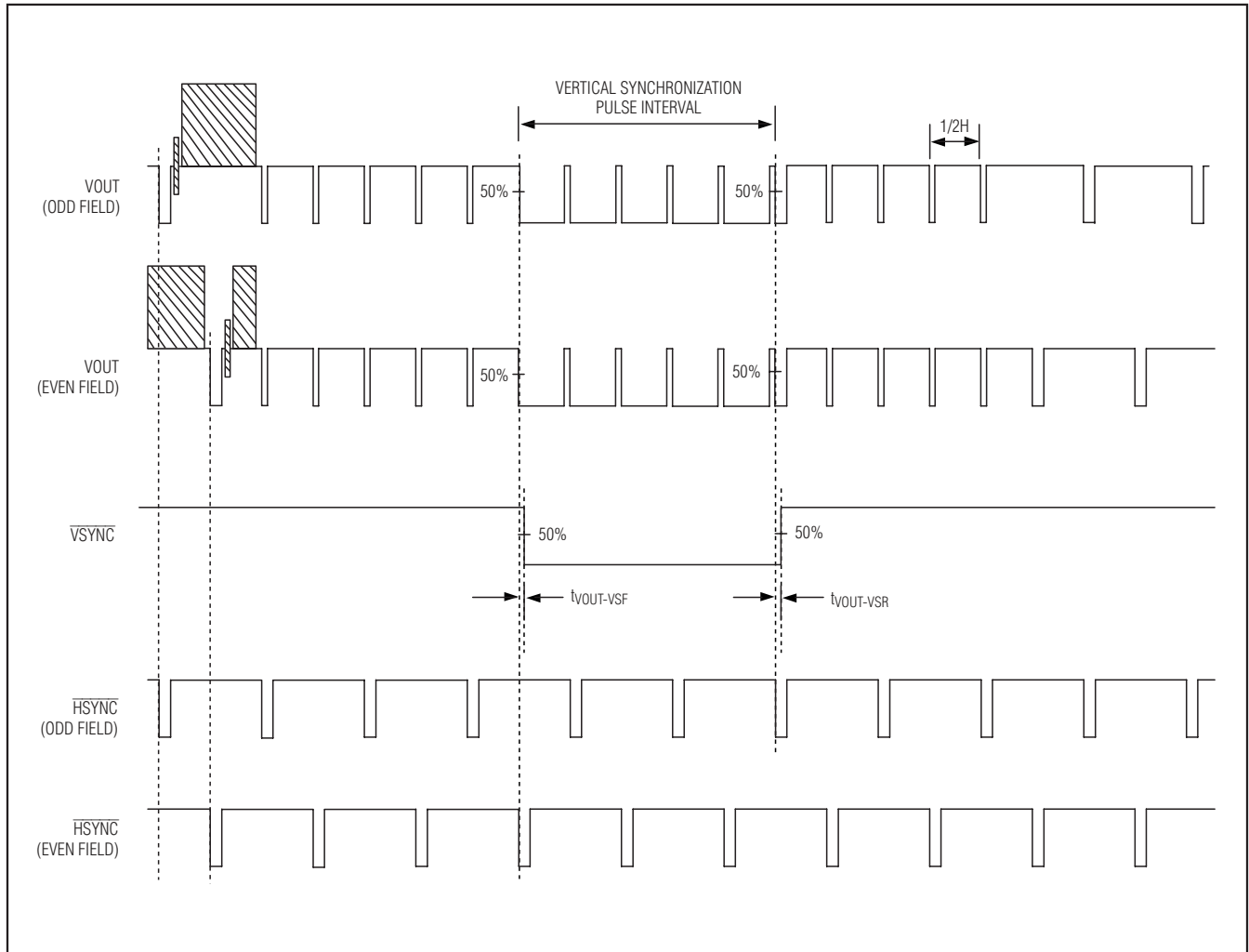
Figure 6. VOUT, \overline{\text{VSYNC}} , and \overline{\text{HSYNC}} Timing (PAL, External Sync Mode)
