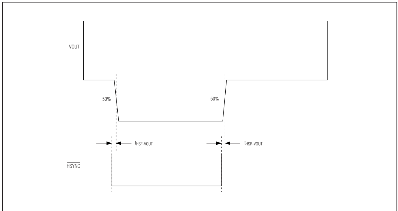
Figure 9. VOUT and \overline{\text{HSYNC}} Horizontal Sync Timing (NTSC and PAL, Internal Sync Mode)
