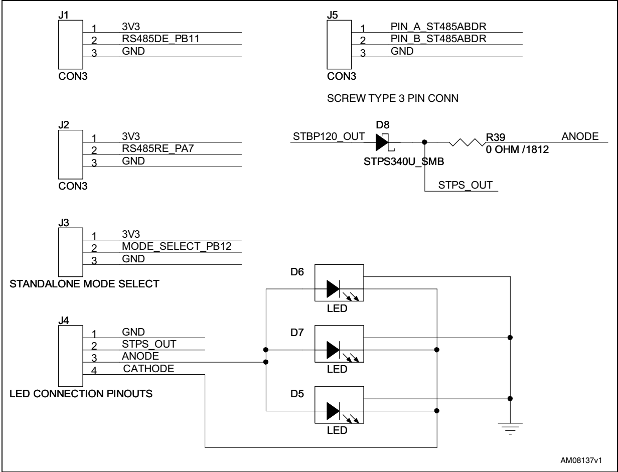
Figure 9. Jumpers
