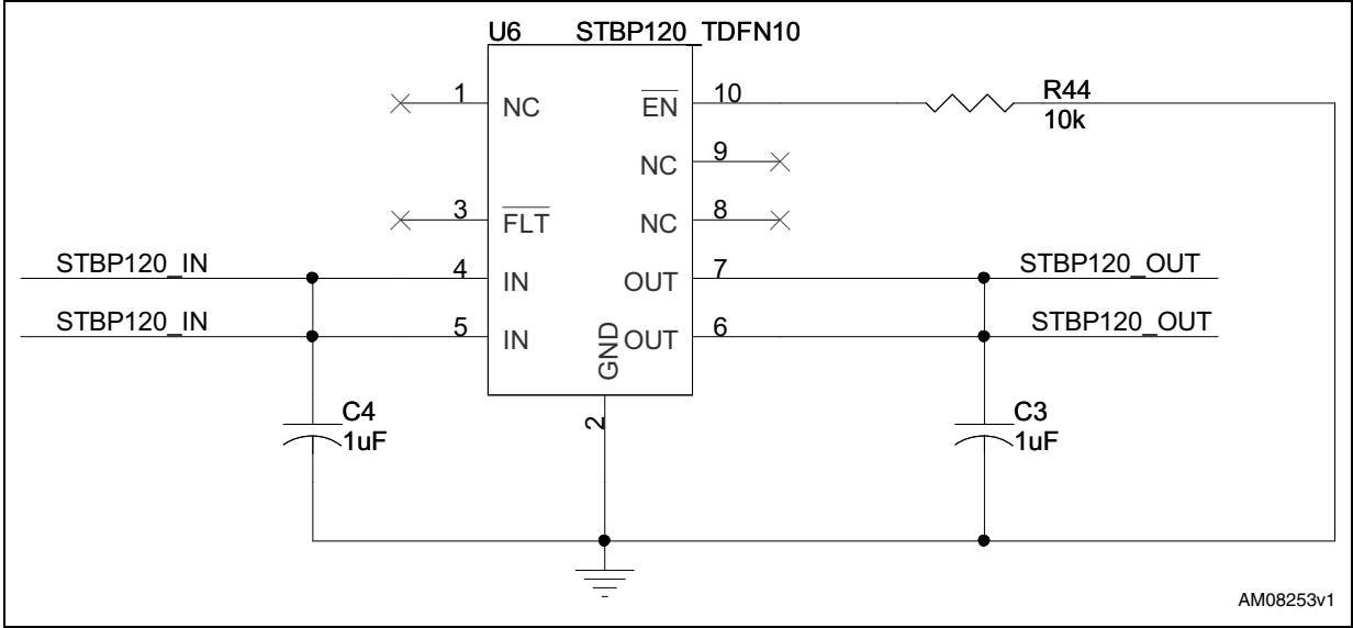
Figure 8. STBP120 section
