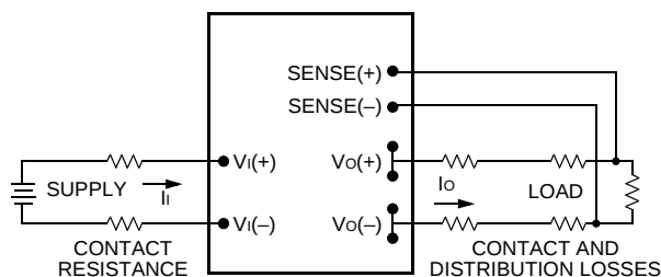
Figure 53. Effective Circuit Configuration for Single-Module Remote-Sense Operation Output Voltage.
