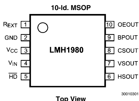
FIGURE 1. Pinout
