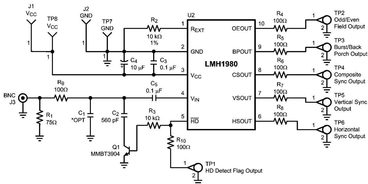
FIGURE 2. Test Circuit
