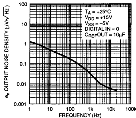
V_{OUT} Noise Density vs. Frequency
