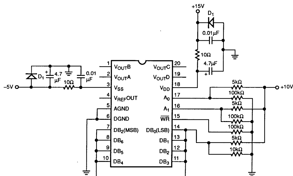
Burn-In Circuit
