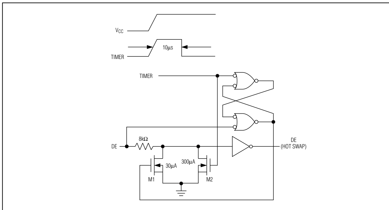
Figure 8. Simplified Structure of the Driver Enable Input (DE)
