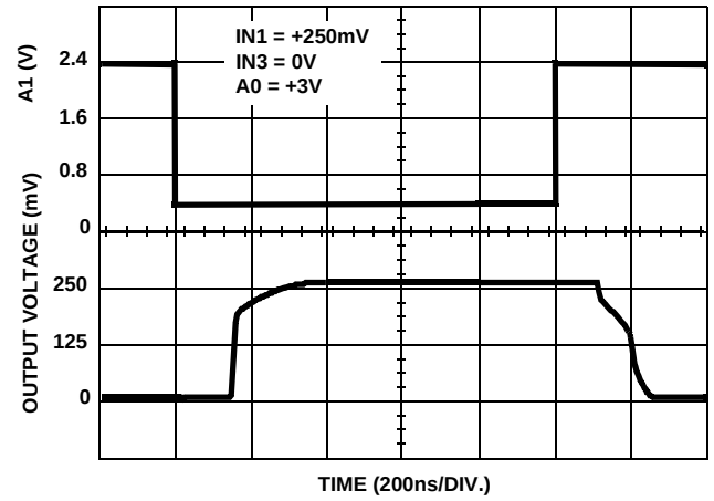
FIGURE 4. CHANNEL-TO-CCHANNEL SWITCHING RESPONSE
