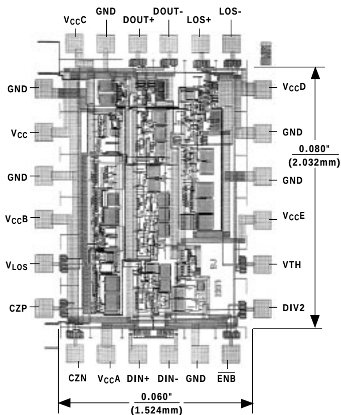
Chip Topography
