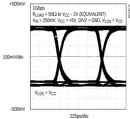
EYE DIAGRAM
