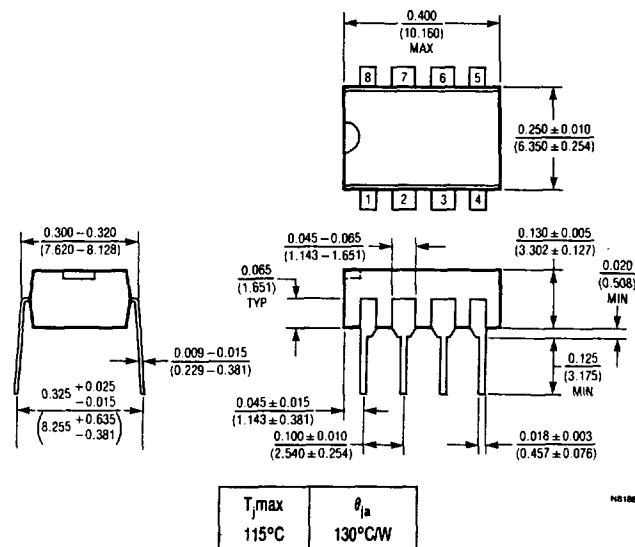
N Package 8 Lead Molded Dip
