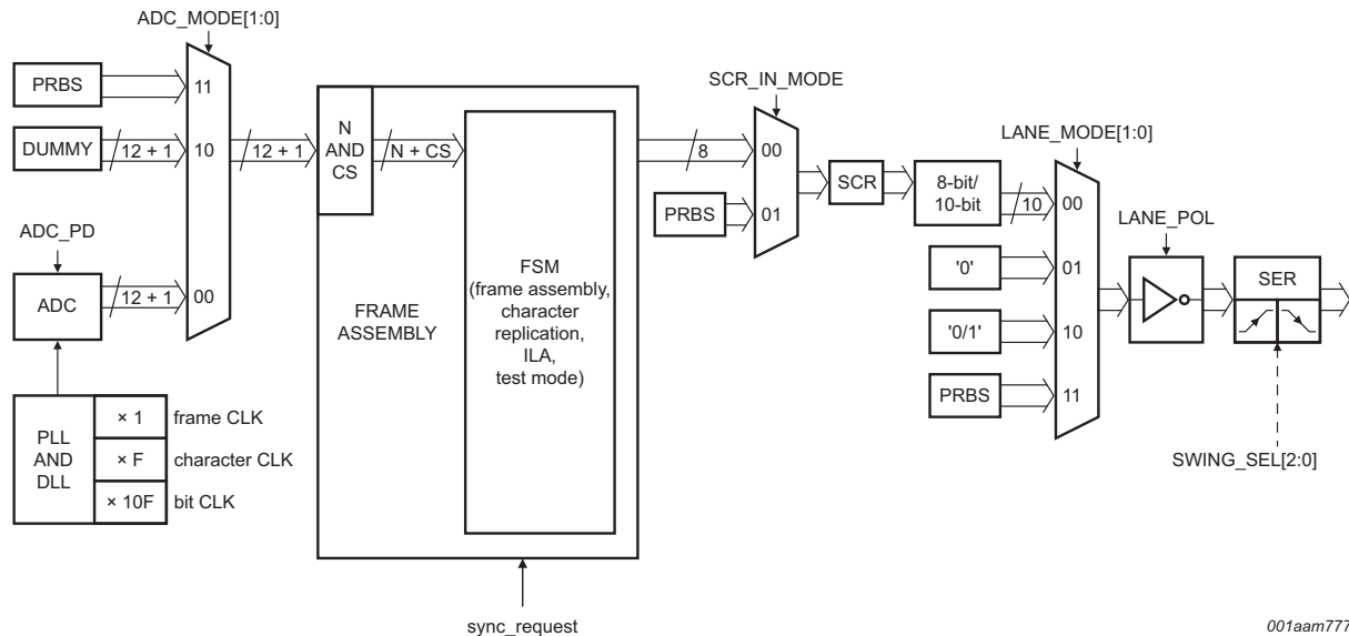
Fig 22. Detailed view of the JESD204A serializer with debug functionality
