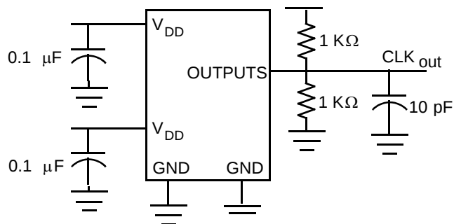
Figure 8. Test Circuit 2
