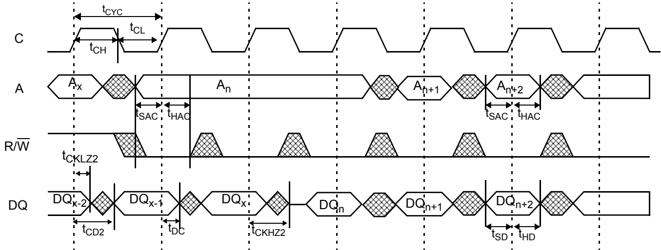
Figure 27. READ-to-WRITE for Pipelined Mode ( \overline{\text{OE}} Controlled) [62, 63]
