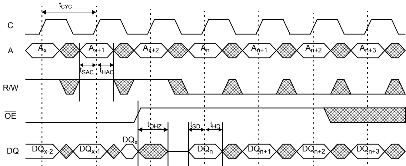
Figure 27. READ-to-WRITE for Pipelined Mode ( \overline{\text{OE}} Controlled) [62, 63]
