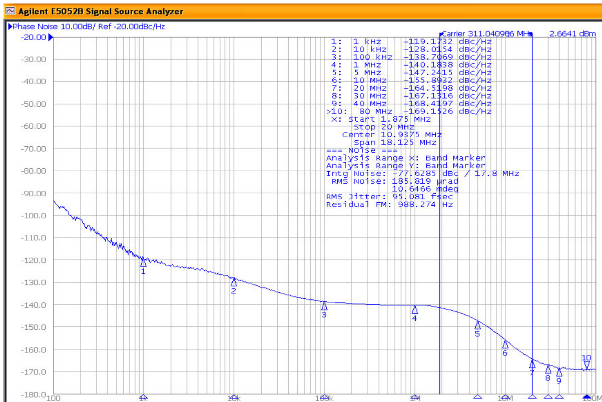
Figure 1. HCSL Output 311.04MHz 1.875MHz-20MHz 95fs
