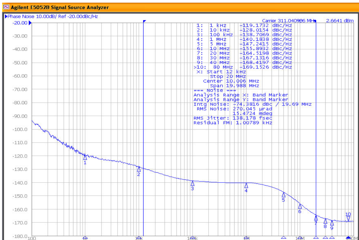
Figure 2. HCSL Output 311.04MHz 12kHz-20MHz 138fs
