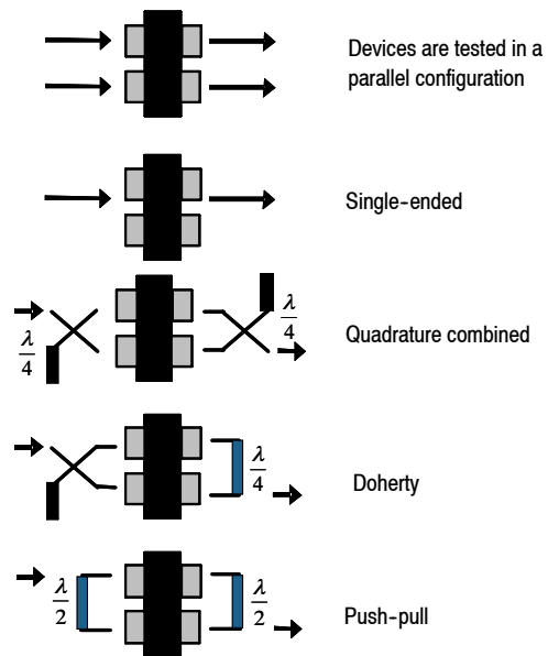
Figure 3. Possible Circuit Topologies
