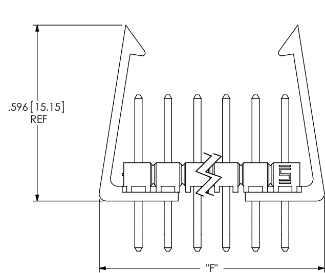
FIG 2 (TSW-1XX-XX-XX-S-LC SHOWN) (SAME AS FIG 1, DIFFERENT AS SHOWN)
