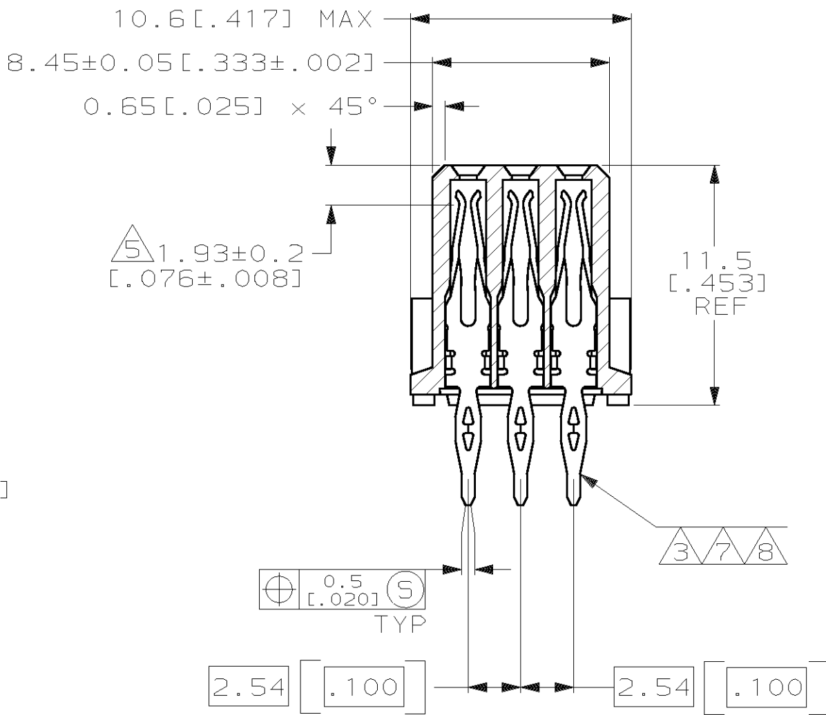
SECTION X-X
