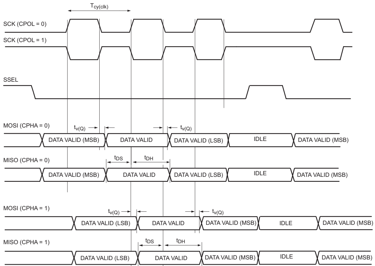
Fig 22. SPI master timing
