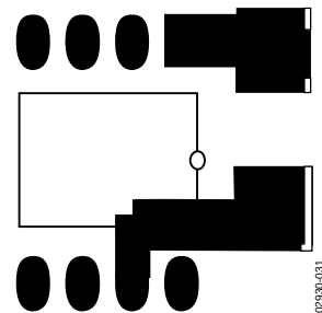
Figure 32. Recommended Supply Decoupling Scheme for the AD7476A/AD7477A/AD7478A MSOP Package
