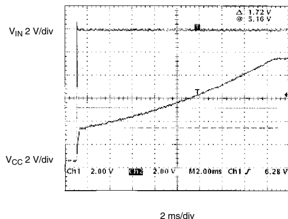
Figure 12. V_{CC} Ramp-Up
