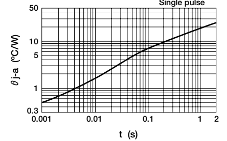
\theta_{JA} — t Characteristics
