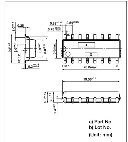
External Dimensions SMD-16A
