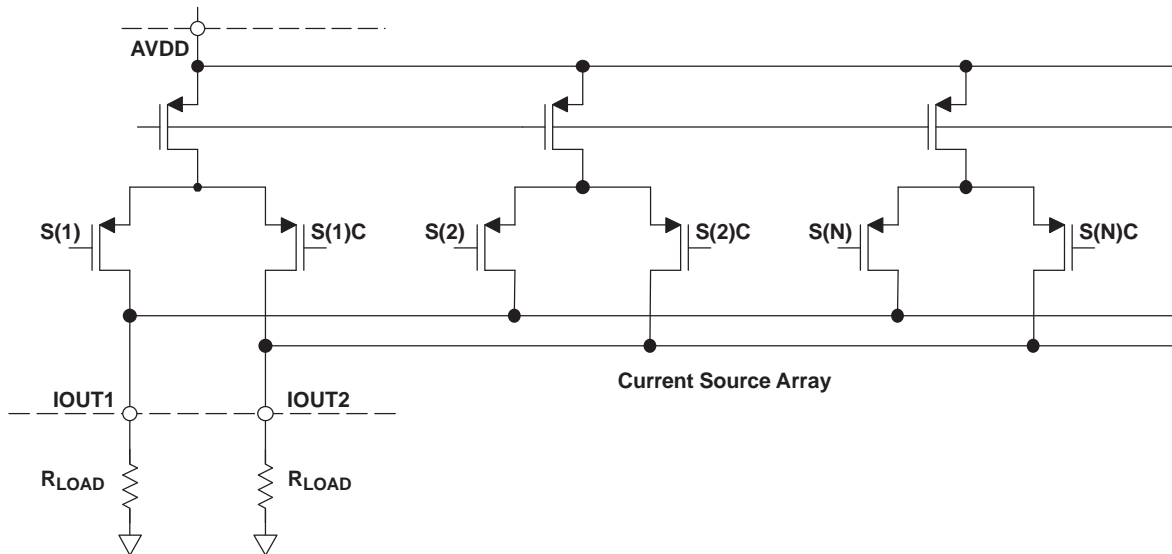
Figure 20. Analog Outputs
