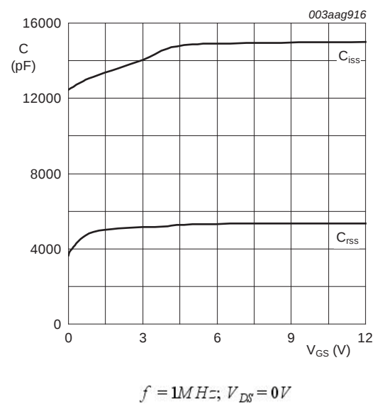
Fig 17. Input and reverse transfer capacitances as a function of gate-source voltage, typical values
