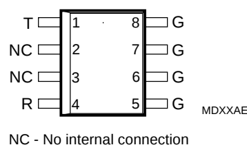
D PACKAGE (TOP VIEW)
