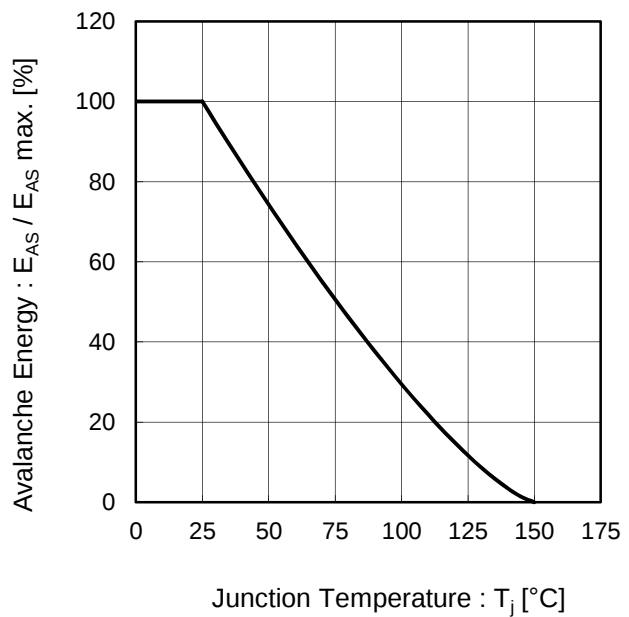
Fig.4 Avalanche Energy Derating Curve vs Junction Temperature
