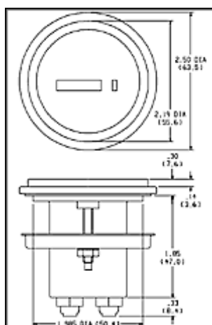
Chrome Flush Mount (Cup) 2.5": Panel cutout 2.00 diameter opening. *
