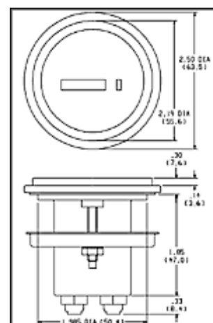
Black Flush Mount (Stirrup) 2.5": Panel cutout 2.00 diameter opening. *
