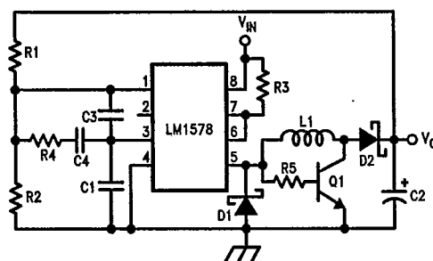
FIGURE 9. Buck-Boost Regulator
