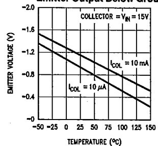
Collector Current With Emitter Output Below Ground
