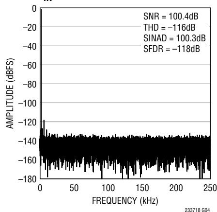
32k Point FFT f_s = 500\text{kpsps} , f_{IN} = 2\text{kHz}
