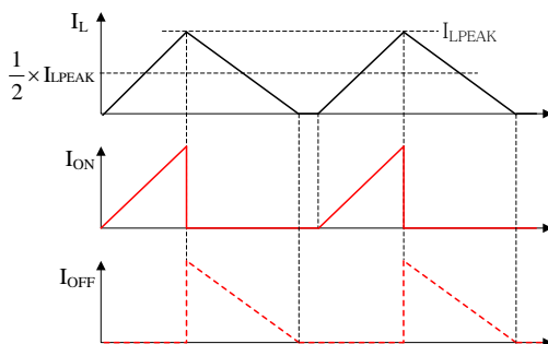
Figure 8-2 Operational waveform of single phase DCM
