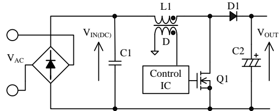
Figure 8-8 General current detection circuit of single phase PFC
