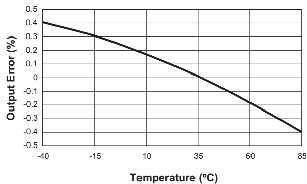
Output Voltage Error vs. Temperature ( V_{IN} = 3.6V; V_{OUT} = 12V; I_{OUT} = 100mA )
