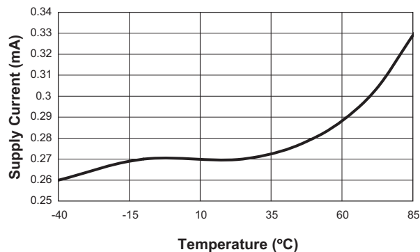
No Load Input Current vs. Temperature ( V_{IN} = 3.6V; V_{OUT} = 5V )
