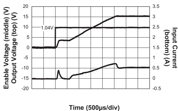
Soft Start
