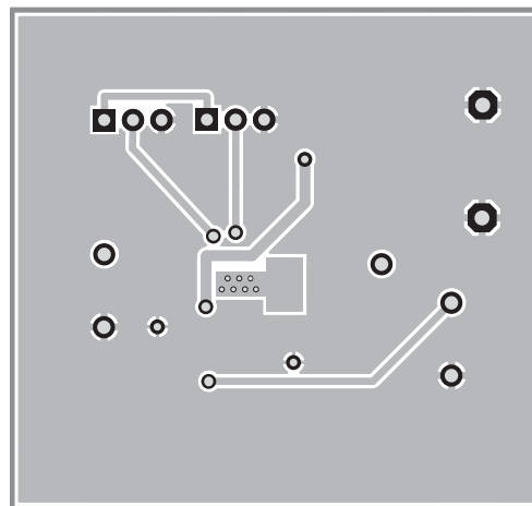
Figure 7: AAT1210 Evaluation Board Bottom Side Layout.
