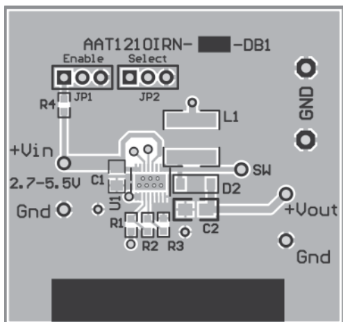
Figure 6: AAT1210 Evaluation Board Top Side Layout.
