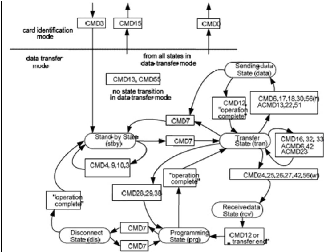
Figure 6-29: microSD Card state diagram (data transfer mode)
