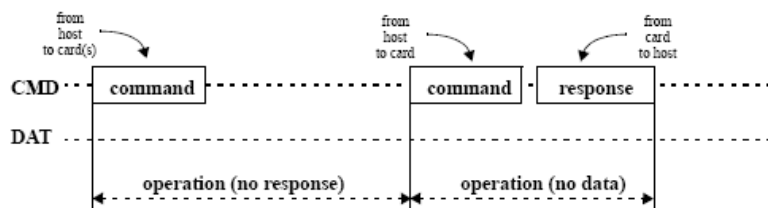
Figure 6-1: “no response” And “no data” Operations
