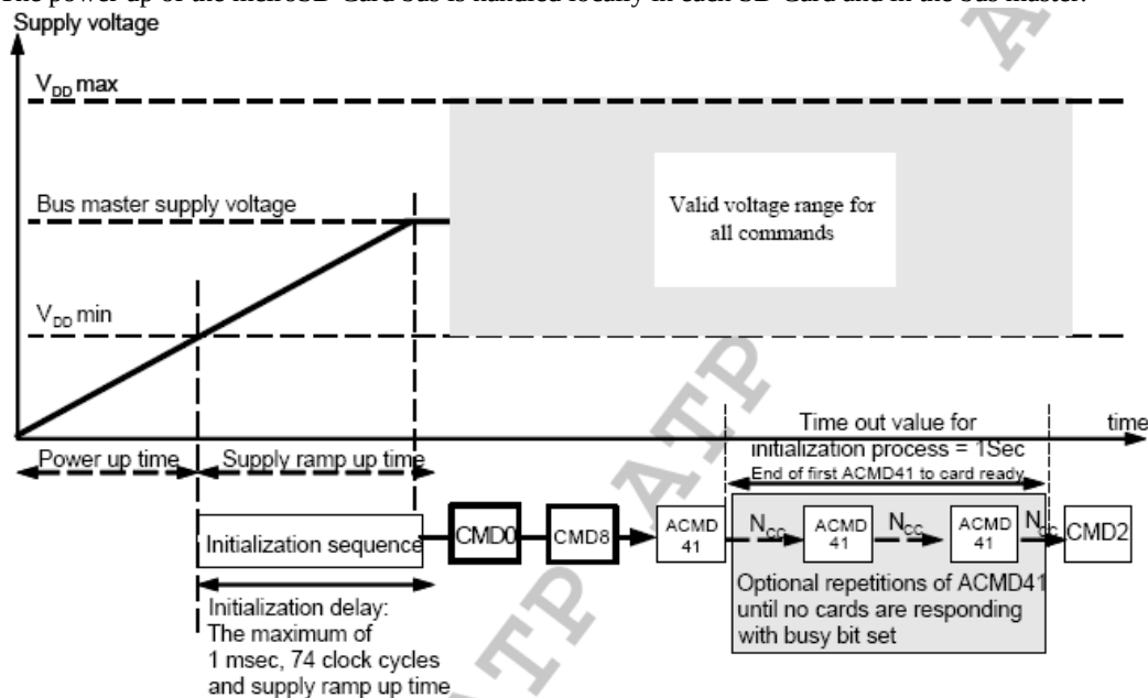
Figure 4-4: Power-up diagram
