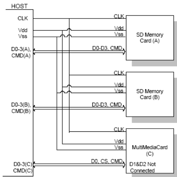
Figure 4-2: mcirioSD Card system bus Topology
