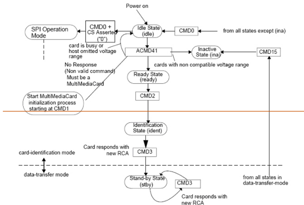
Figure 6-827: microSD Card state diagram (card identification mode)
