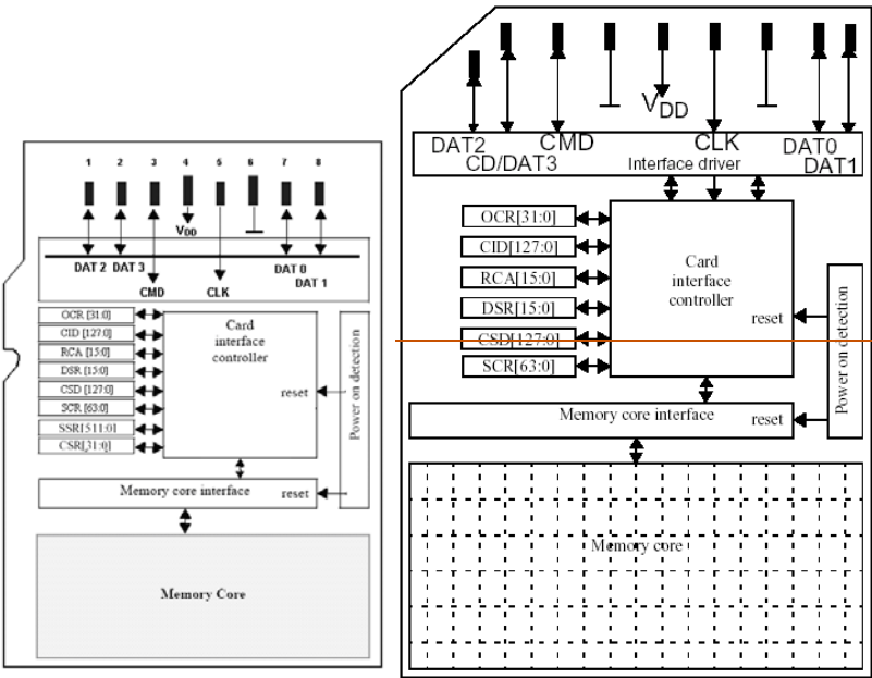
Figure 4-1: microSD Card Function Block Diagram
