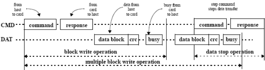
Figure 6-3: (Multiple) Block Write Operation
