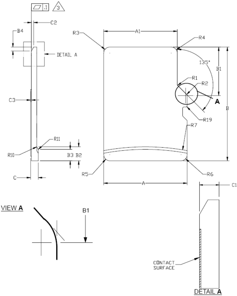
Figure 12-12: Dimensions Of microSD (Top View)
