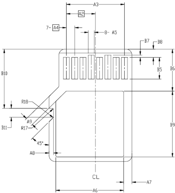
Figure 12-11: Dimensions of microSD (Bottom View)
