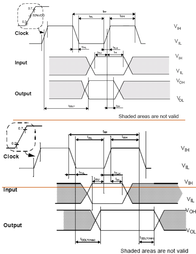
Figure 3-2: Timing diagram data input/output referenced to clock (Default)
