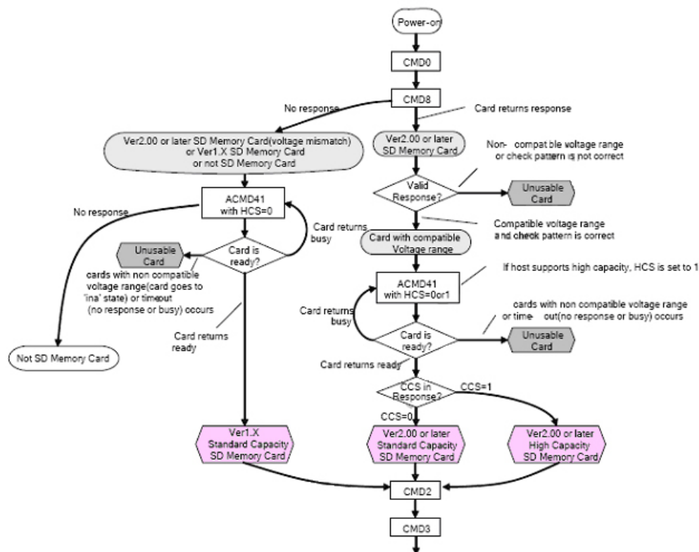
Figure 6-828: Card Initialization and Identification Flow (SD mode)
