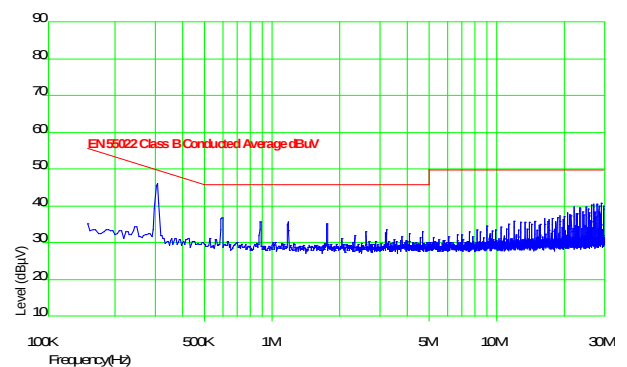
Figure 68. EMC signature using above filter, HW005A0F.
