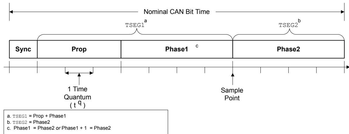
Figure 12-4. CAN Bit Time
