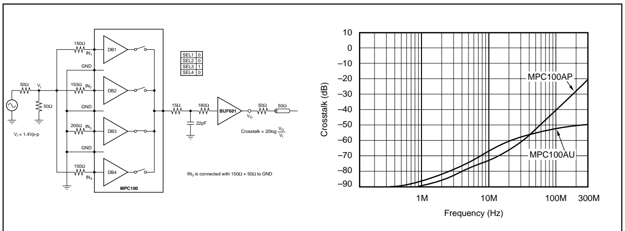
FIGURE 4. Channel Crosstalk— 150\Omega Input Resistor.
