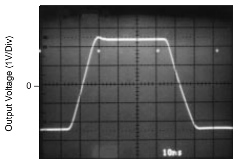
LARGE SIGNAL PULSE RESPONSE
