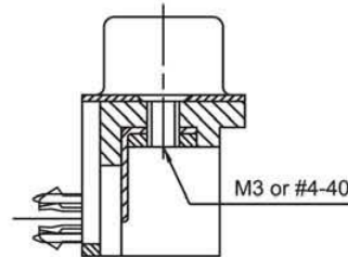
Threaded Rear Insert 4R / 3R
