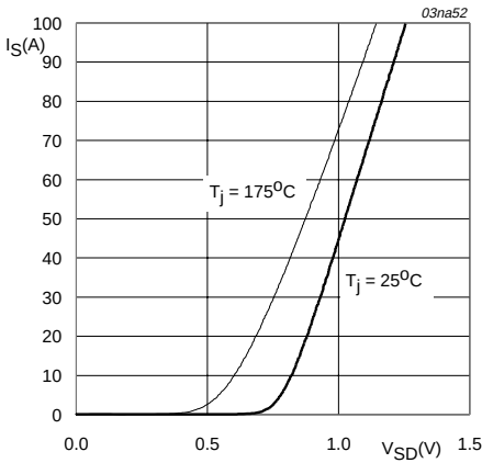
Fig 15. Reverse diode current; typical values.
