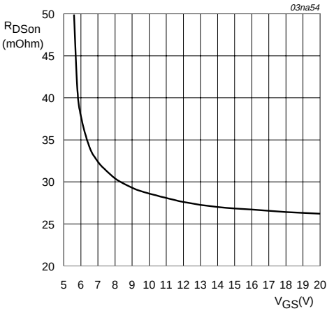
Fig 6. On-state resistance: typical values.
