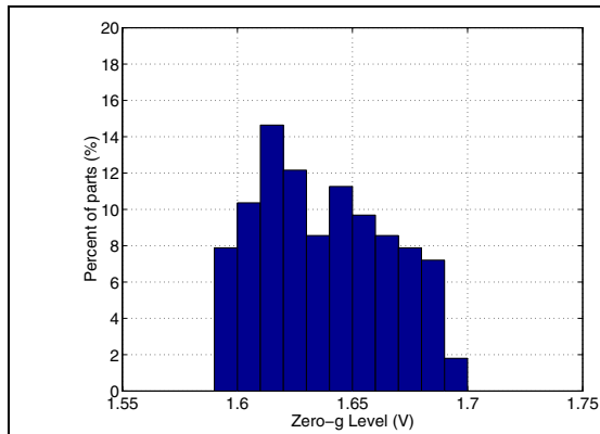
Figure 7. y-axis Zero-g level at 3.3V
