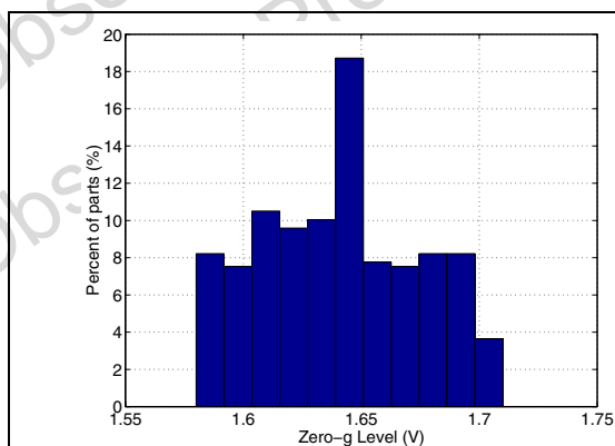
Figure 9. z-axis Zero-g level at 3.3V
